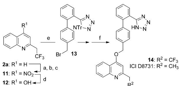
Scheme 3. Synthesis of trifluoromethylated analogue of ICI D8731.
